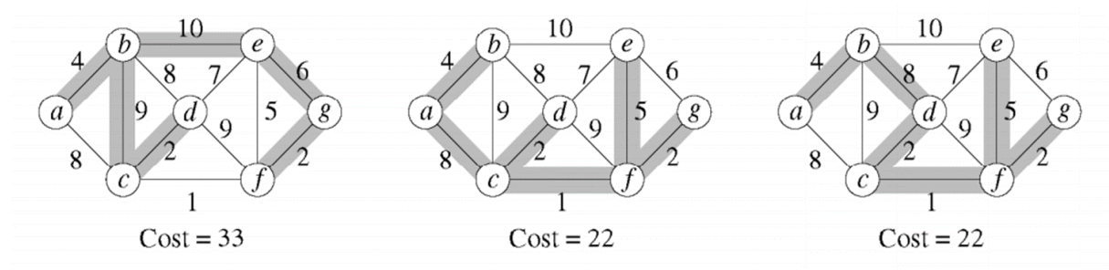
Figura 63: minimal spanning tree
