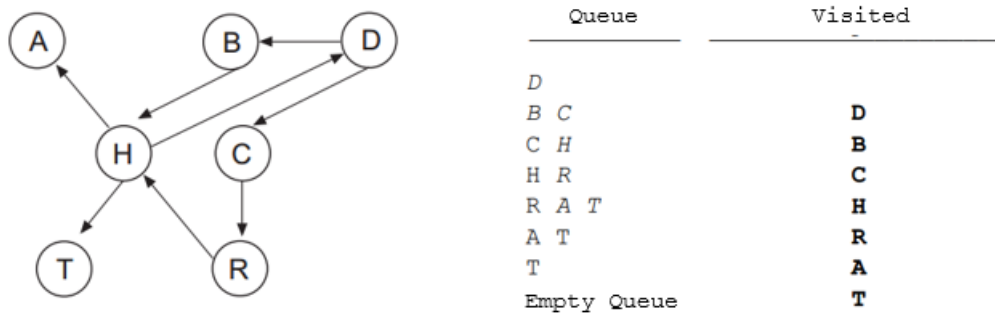
Figura 55: breadth first alg
